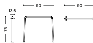
PALISSADE MIDDLE LEG LENGTH 90 CM | 35.50" DEPTH 13,5 CM | 5.25" HEIGTH | 75 CM | 29.50"
